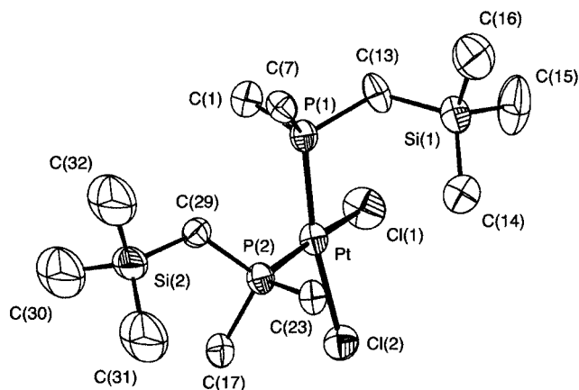
Figure 1. ORTEP drawing of the molecular structure and numbering scheme of 4
