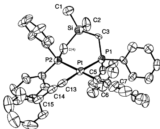
Figure 3. ORTEP drawing of the molecular structure and numbering scheme of 6
