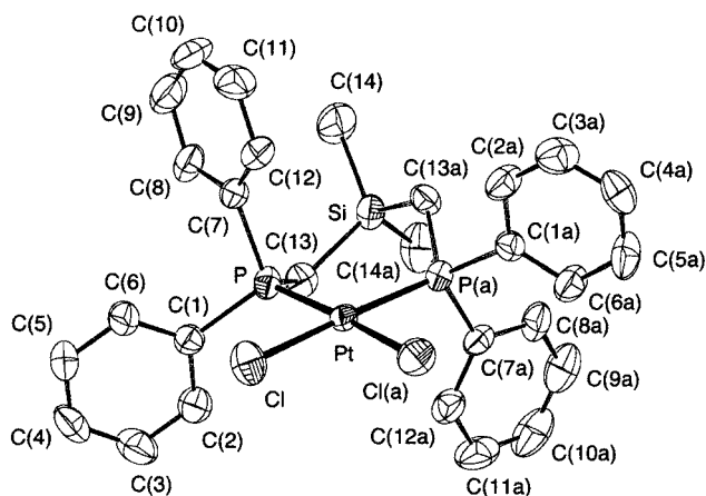
Figure 2. View of the molecular structure of 5 together with the atomic numbering scheme
